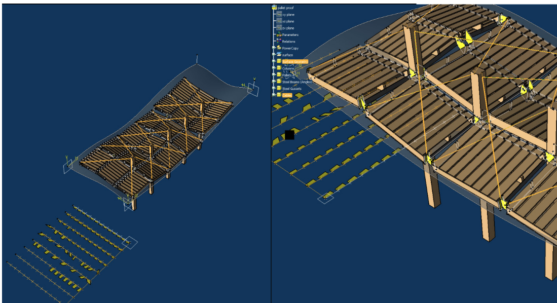
Figure 2- "Quilt" of pallets in Gehry Technologies
