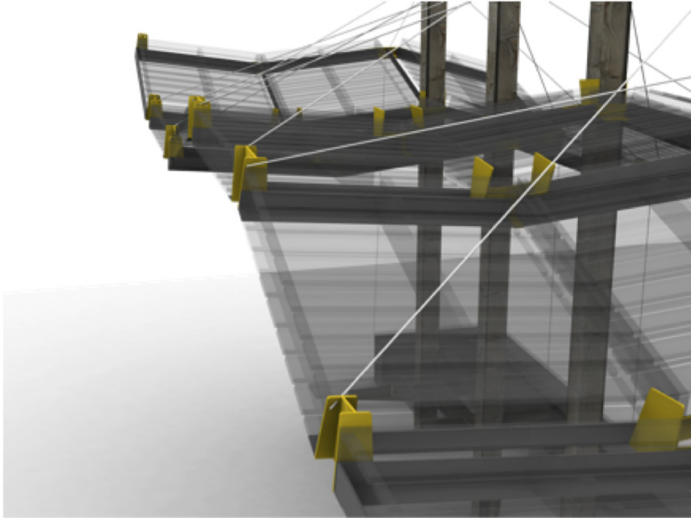
Figure 4- model detail showing custom components (in yellow)
